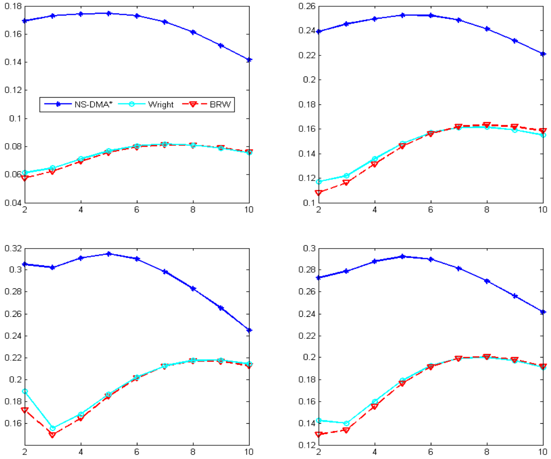
Figure 11: Statistical Evaluation
