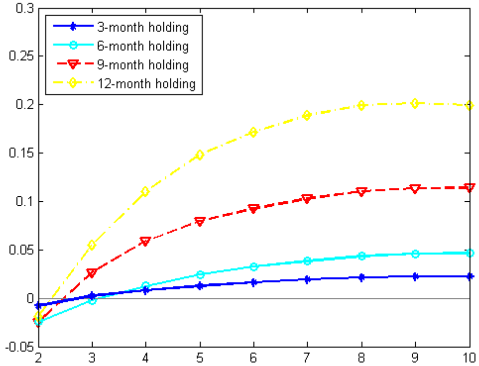
Figure 14: Economic Evaluation
