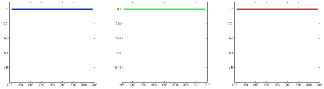
Figure 9: DPS results
