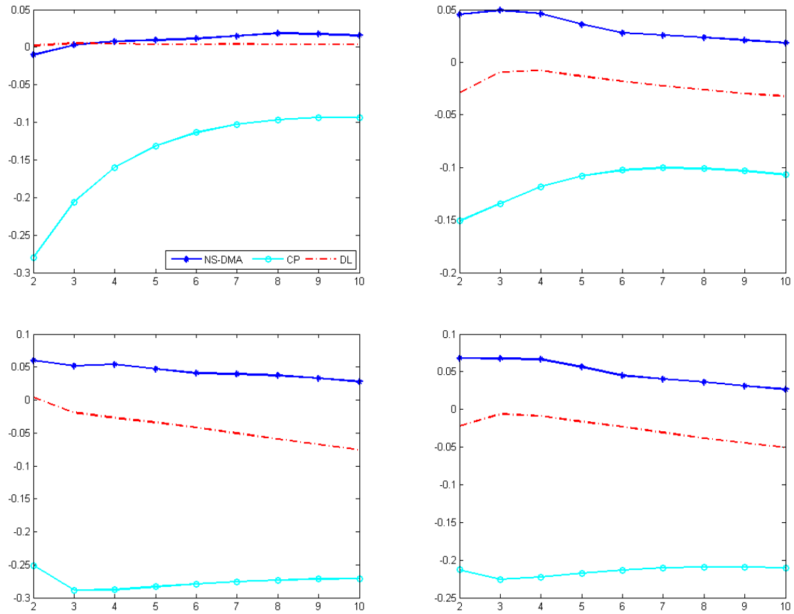
Figure 13: Statistical Evaluation
